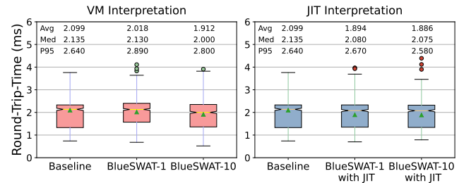
Figure 5: RTT (ms) in end-to-end micro benchmark.
